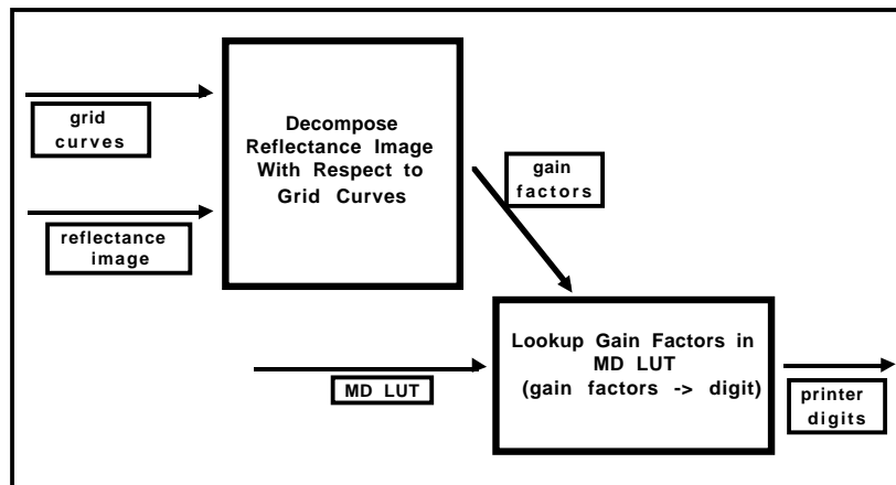
Figure 9: Image processing with spectral lookup method. Each reflectance image pixel is decomposed into gain factors associated with the grid curves. The lookup table constructed in Figure 8 expects these values as input and reports printer digits.
