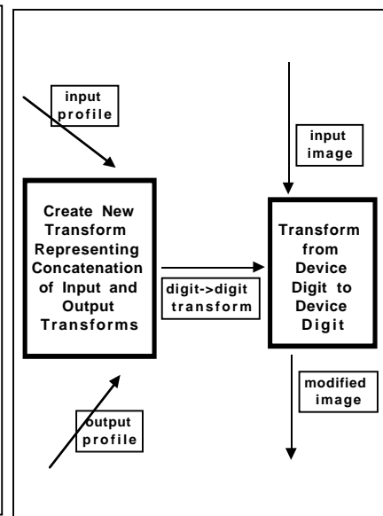
Figure 1c: Typical ICC image processing with efficiencies. Transform box may include 1-D and 3-D lookups and matrices.
