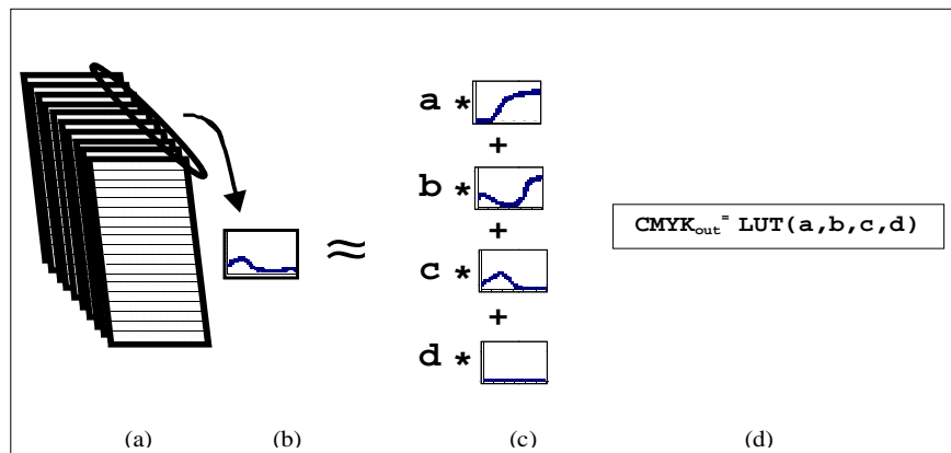
Figure 6: Reduction of dimensionality, starting with a 31- to 4-dimensional problem and reducing it to a 4- to 4-dimensional problem. (a) 31 input bands. (b) Each pixel represents 31 samples of a reflectance spectrum. (c) Derive weightings for a set of fixed spectra such that the sum of the weighted spectra is an approximation of the original spectrum. (d) Weights are used as input to a 4- to 4-dimensional lookup table.
