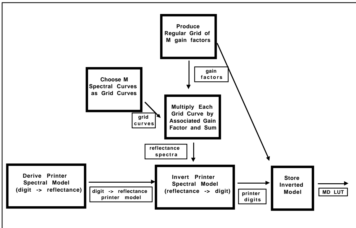
Figure 8: Process for creating a printer characterization for a spectral-based color management system.
