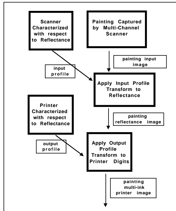
Figure 5: Block diagram illustrating the logical color management system actions which would accompany the painting reproduction example described above. The painting reflectance image is converted to printer digits and then printed.
