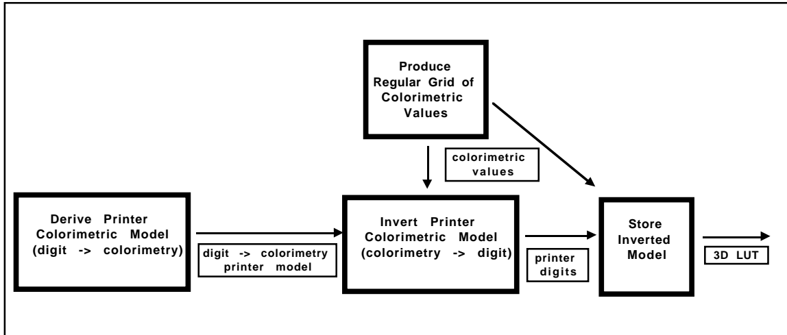
Figure 7: Process for creating a printer characterization for a colorimetric-based color management system.
